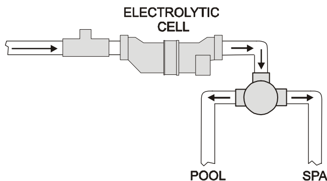
Inverted Installation
